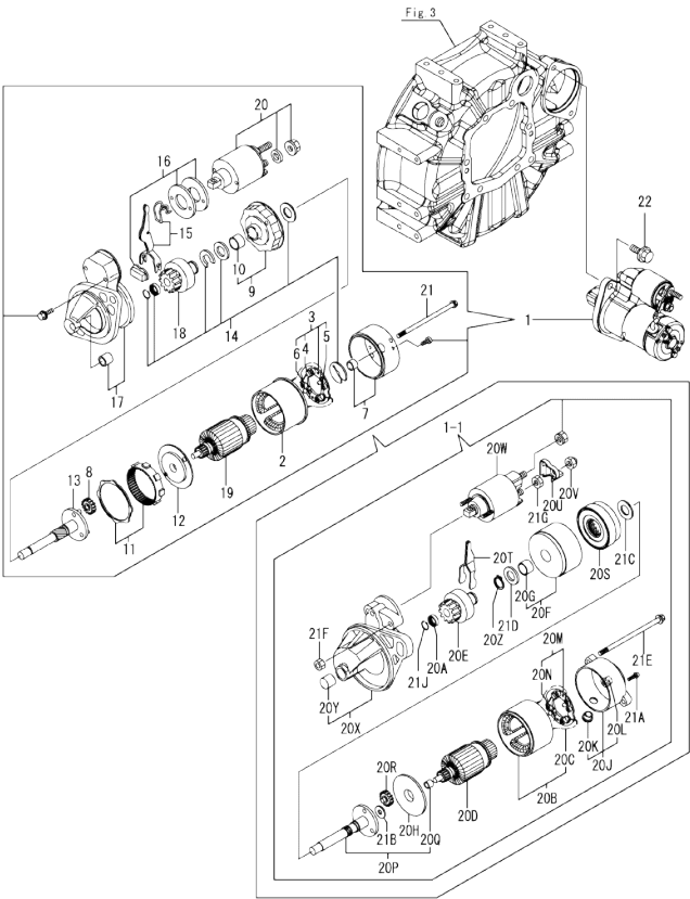
0CW10-M34200 3TNM68-GGE/HGE Fig.14. STARTING MOTOR
