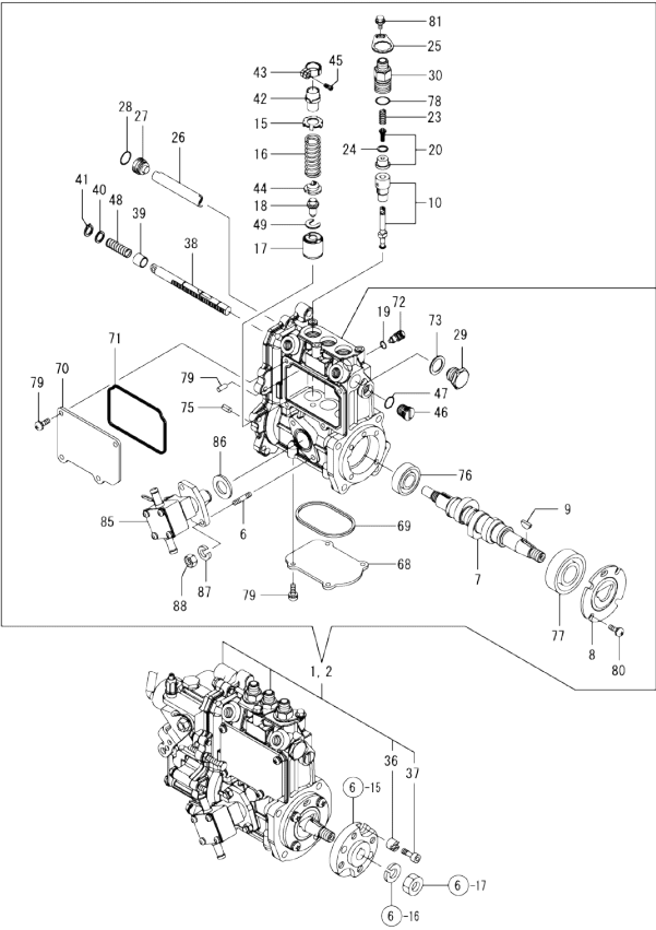
0CW10-M34200 3TNM68-GGE/HGE Fig.10. FUEL INJECTION PUMP
