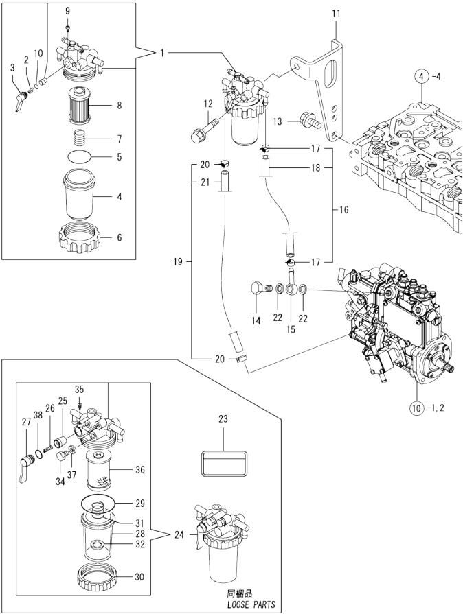
Fig.13. FUEL LINE
